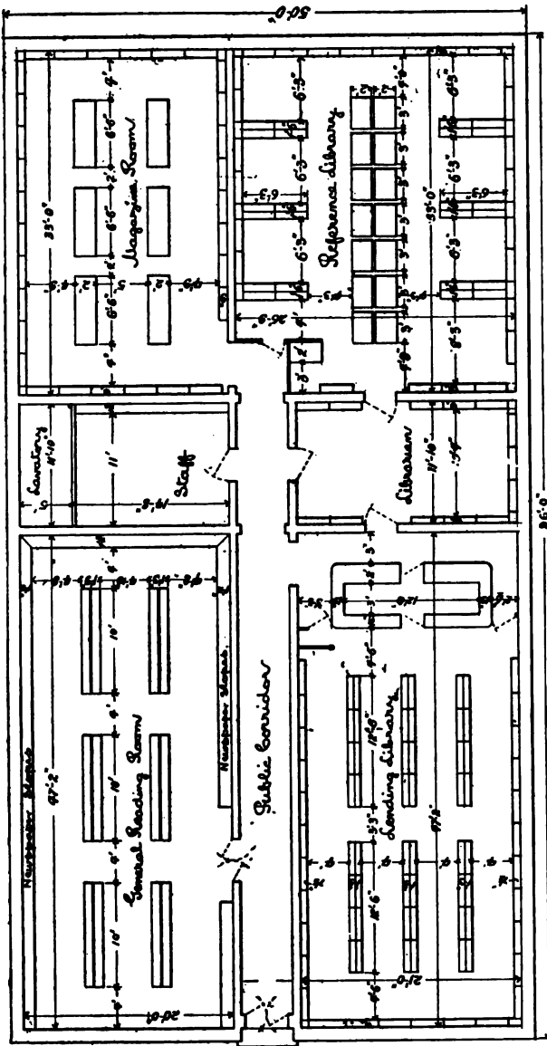
FIG. 16.—Sketch Plan of a Library on one floor (Section 125).
